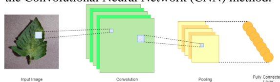
Figure 3. Convolutional Neural Network (CNN) Architecture
